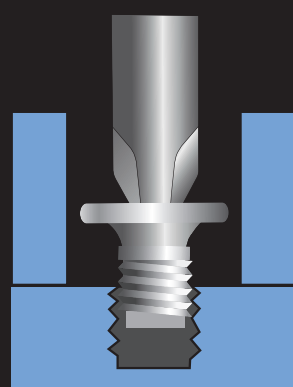
Recessed Screw
