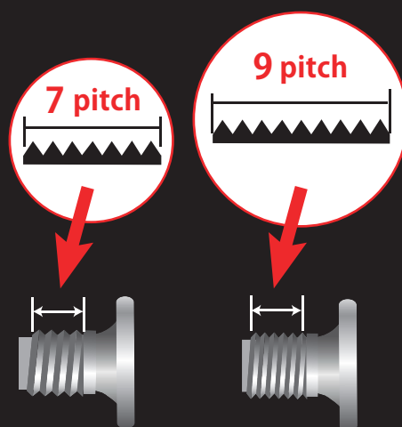
Different Pitch
